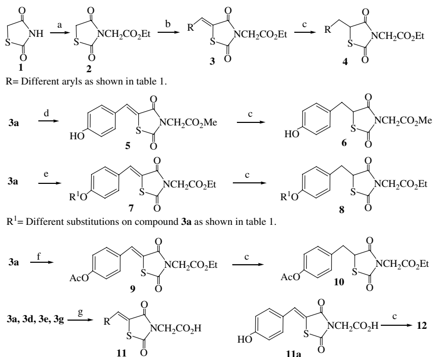
Scheme 1. Reagents: (a) NaH, ethyl bromoacetate, THF; (b) different aldehyde, CH 3 CO 2 H, pyridine, toluene; (c) H 2 –Pd/C, dioxane; (d) H 2 SO 4 , MeOH; (e) XR 1 , K 2 CO 3 , DMF; (f) triethylamine, dichloromethane, AcCl, (g) AcOH, HCl.
